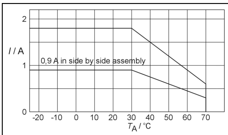
Derating curve for EXO 12CHA.
