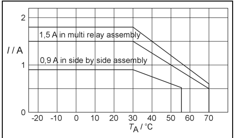
Derating curve for EXO 220CHA.
