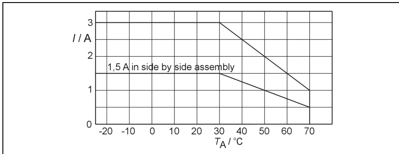
Derating curve for EXO 5CH.
