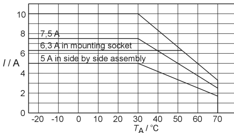
Derating curve for EXO 5CHX.
