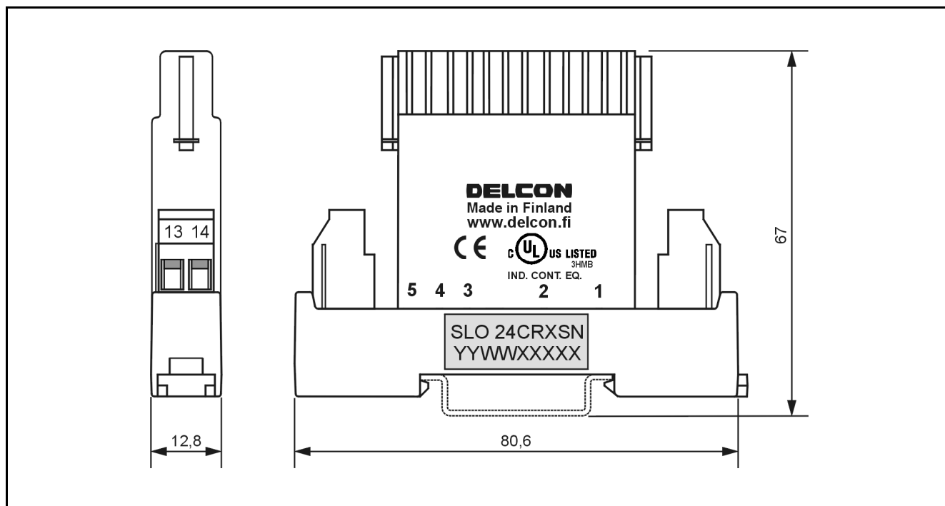
SLO 24CRXSN (dimensions in mm, nominal).
