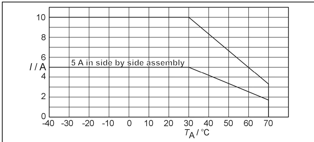
Derating curve for SLO 24CRXSN.
